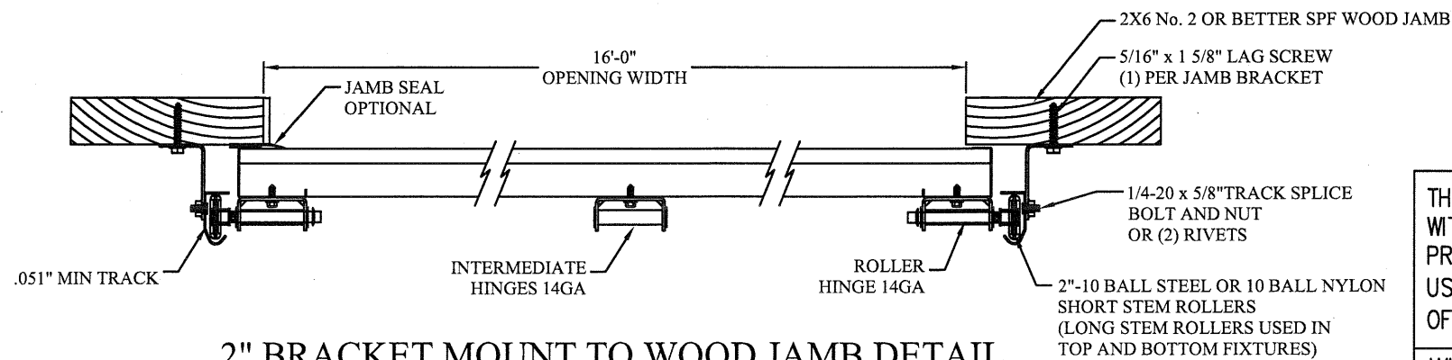
2" BRACKET MOUNT TO WOOD JAMB DETAIL
