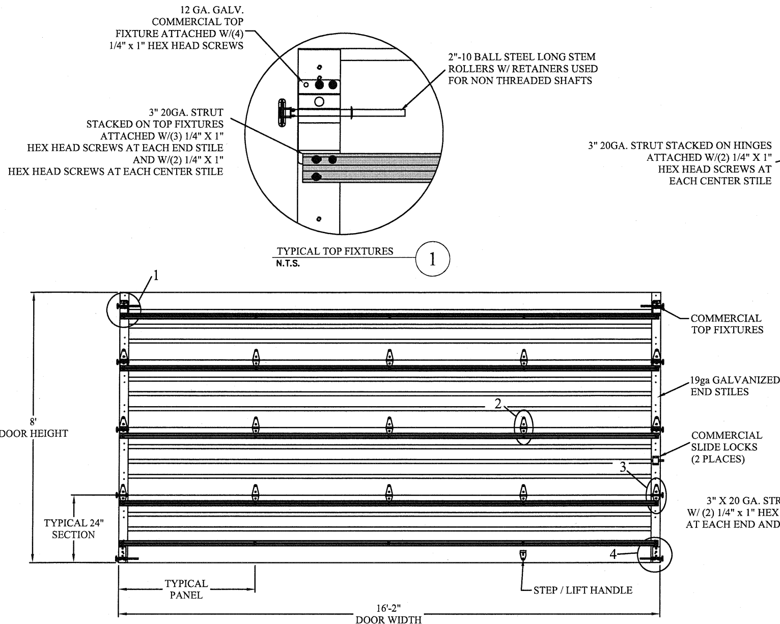
DOOR INTERIOR ELEVATION
